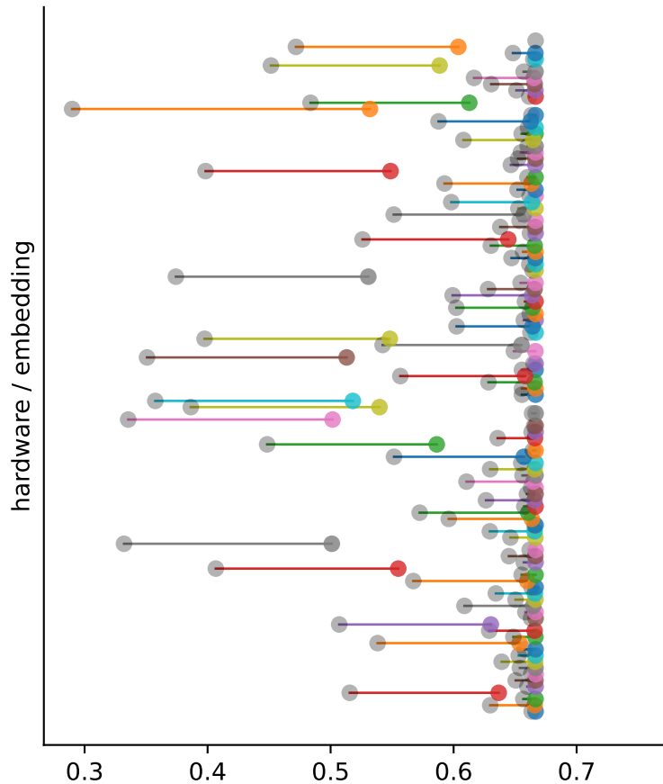
horizon = 2
